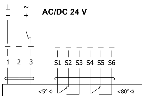
Obr. 3 Servopohon BELIMO BEN 24(-ST)
