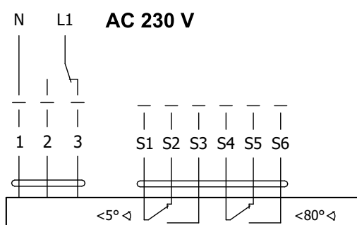
Obr. 8 Servopohon BELIMO BEE 230
